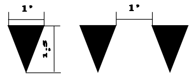
YIELD LINE DETAIL
