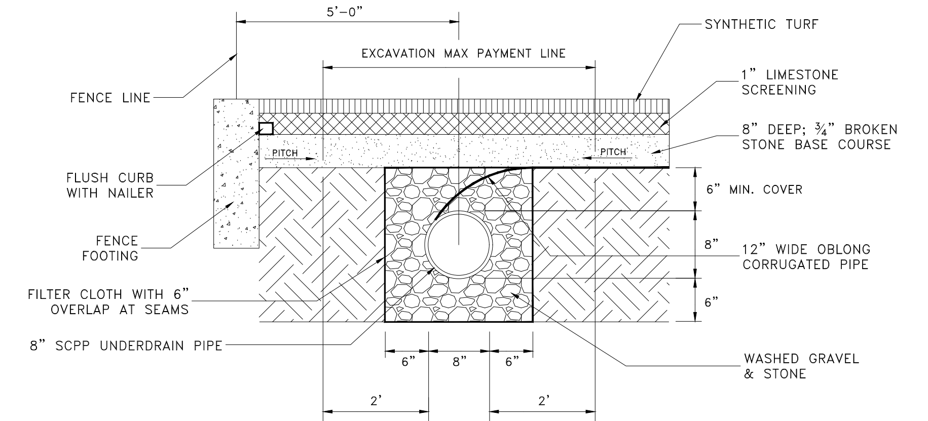
PERIMETER UNDERDRAIN DETAIL ITEM 744 NOT TO SCALE (FLUSH CURB UNDER ITEM 26F)
